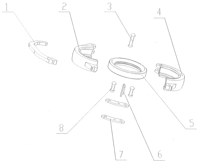
管卡（0019905A0025）Pipe—clip
