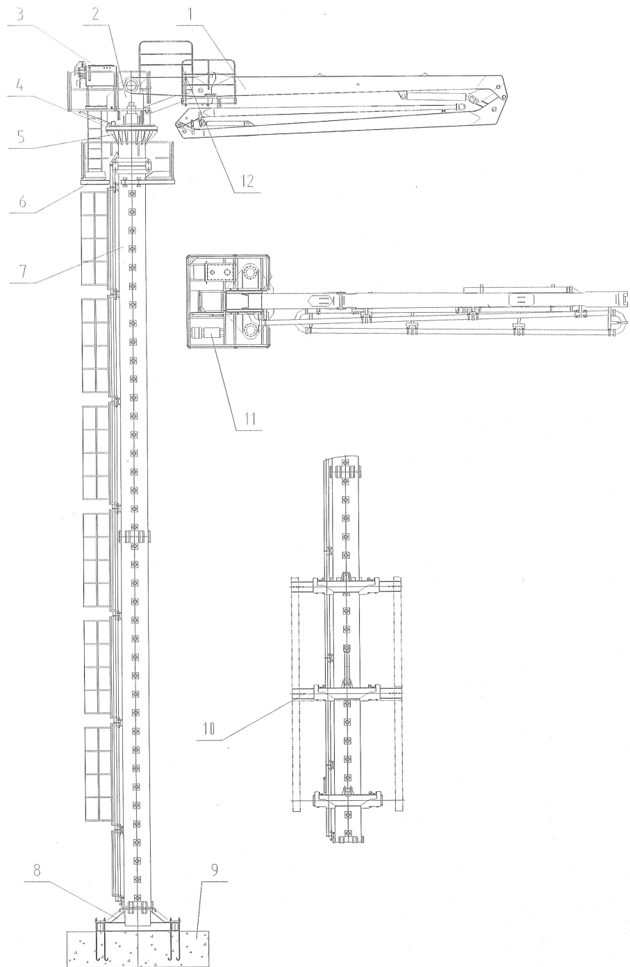
总图 (0050300A2000) General view
